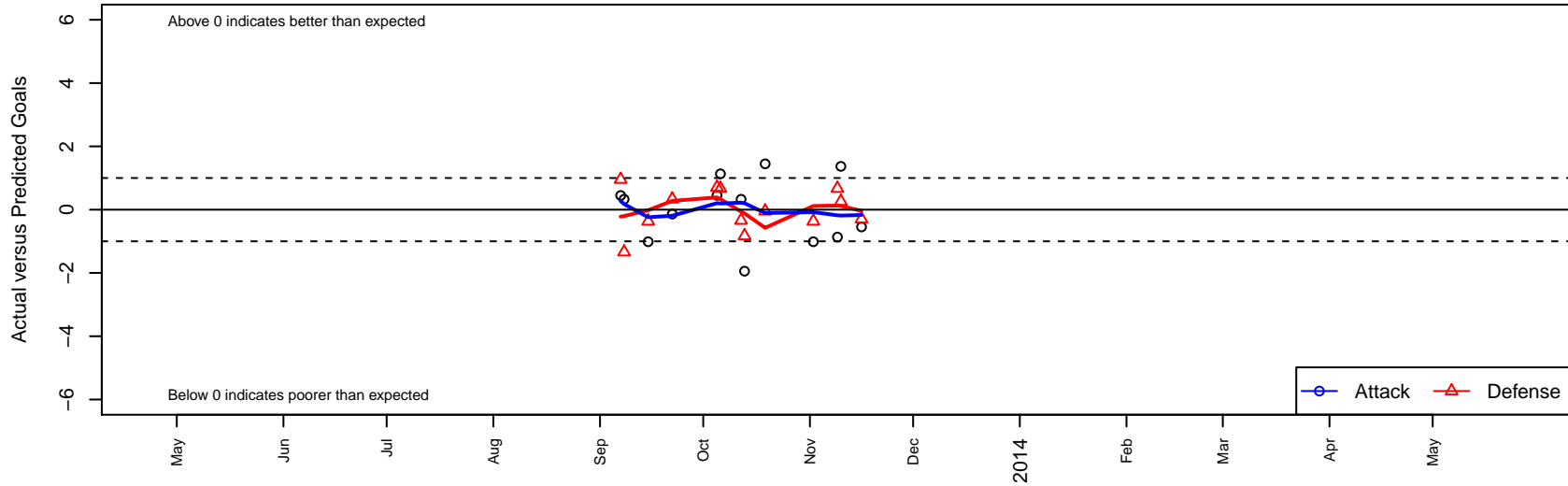
West Coast Wildfire G99 Dots are actual minus expected GF (blue circles) and GA (red triangles). Blue line is smoothed change in attack strength. Red is smoothed change in defense strength.
